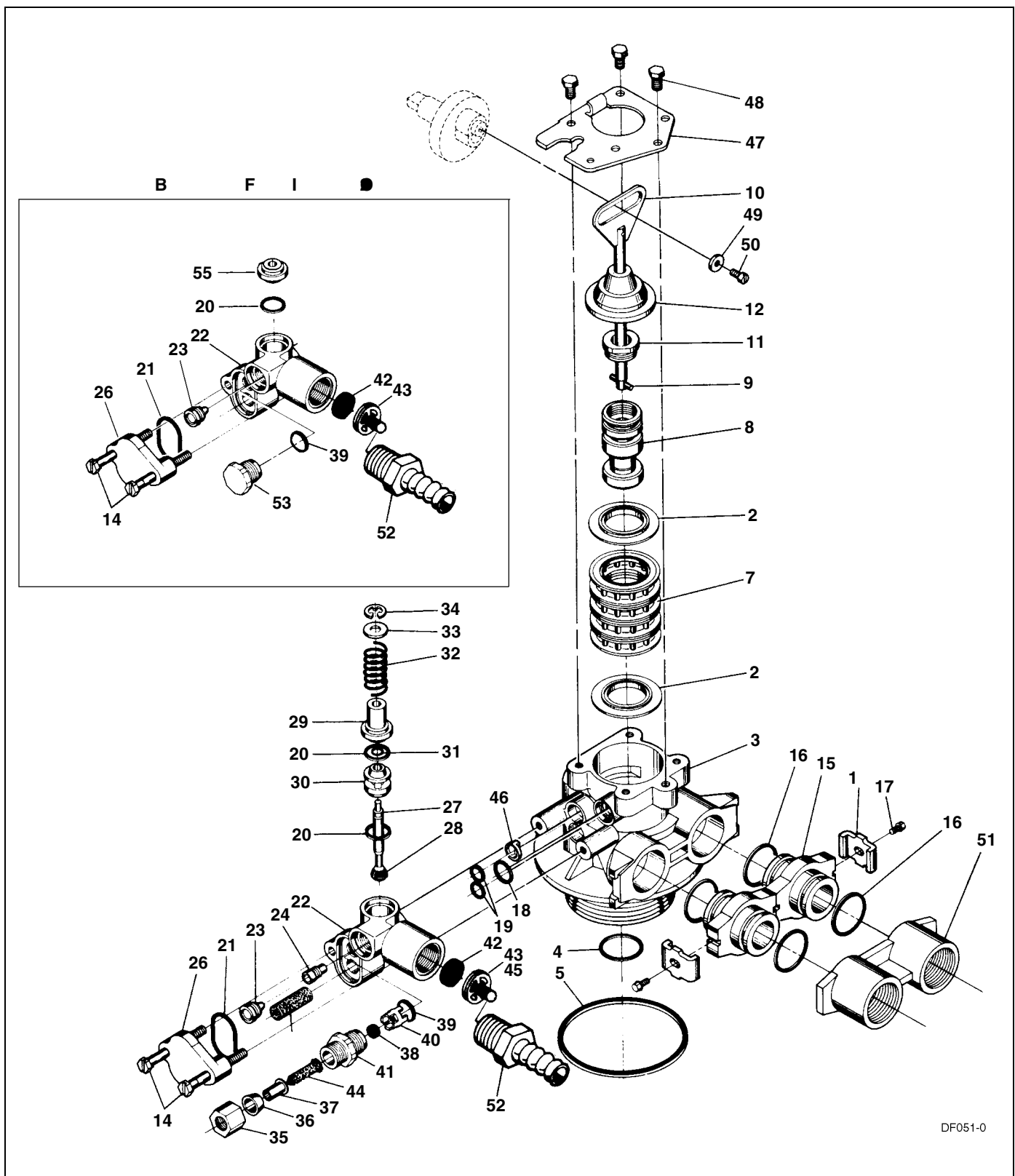
Figure 13: Model 5600 and 5600 E
